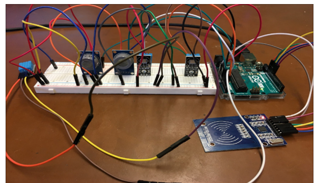
Fig. 2. Arduino microcontroller with temperature-humidity, carbon-monoxide, and RFID sensor.
